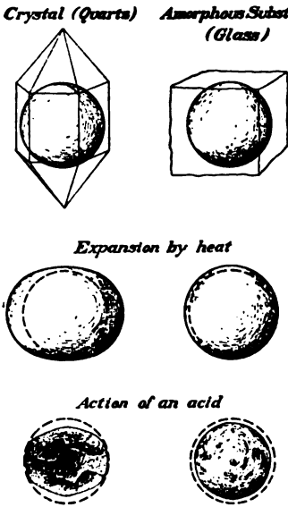
FIG. 10. — Comparison of a crystalline with an amorphous substance when expanded by heat and when attacked by acid.
